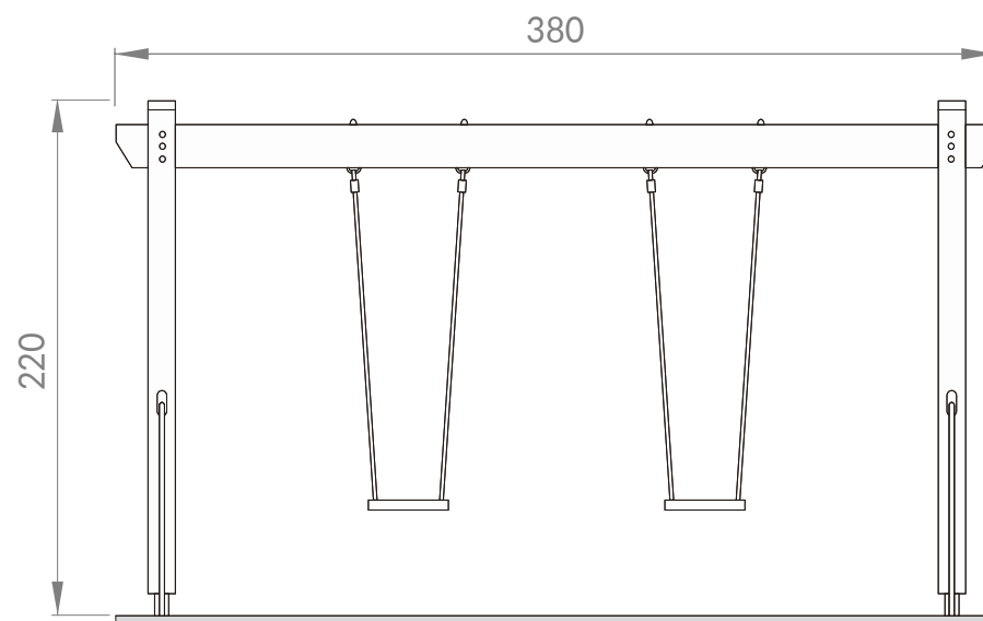
VISTA FRONTAL
