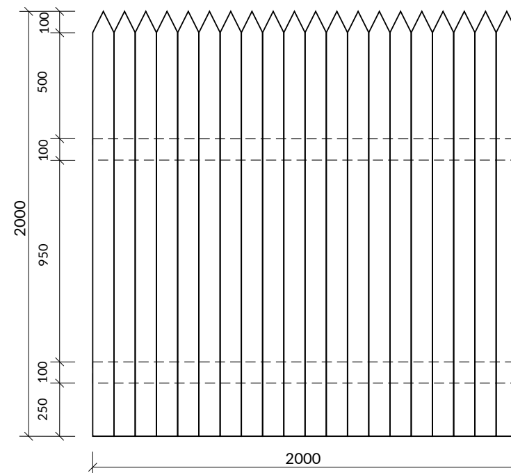
VISTA FRONTAL
