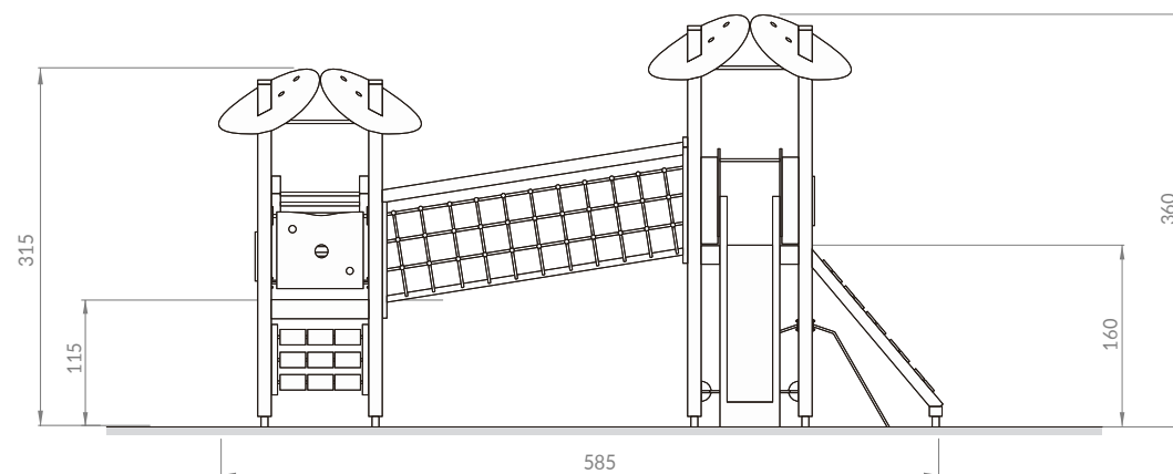
VISTA FRONTAL
